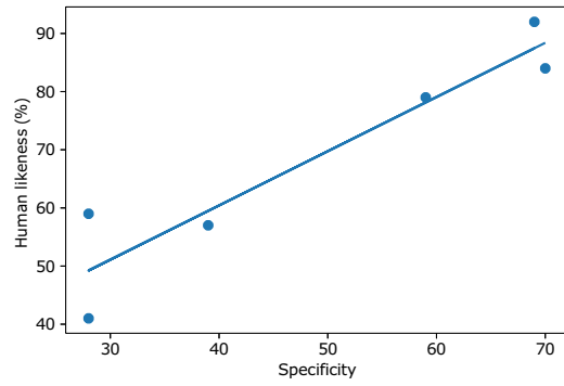
Figure 10: Specificity vs human likeness. Each point is a different chatbot, except for the top right one, which is human. A regression line is plotted, for which the coefficient of determination ( R^2 ) is 0.89, an indication of strong correlation between specificity and human likeness.
