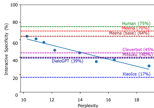
Figure 4: Interactive specificity vs perplexity.
