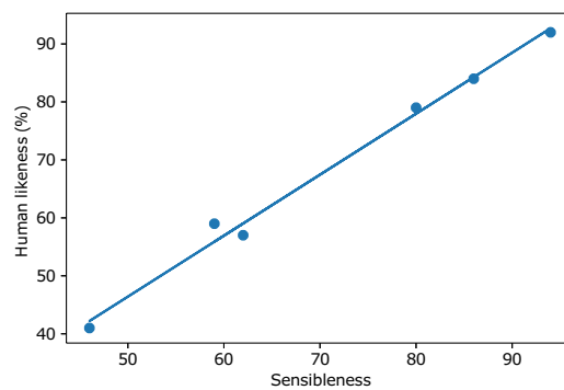
Figure 9: Sensibleness vs human likeliness. Each point is a different chatbot, except for the top right one, which is human. A regression line is plotted, for which the coefficient of determination ( R^2 ) is 0.99, an indication of strong correlation between sensibleness and human likeliness.
