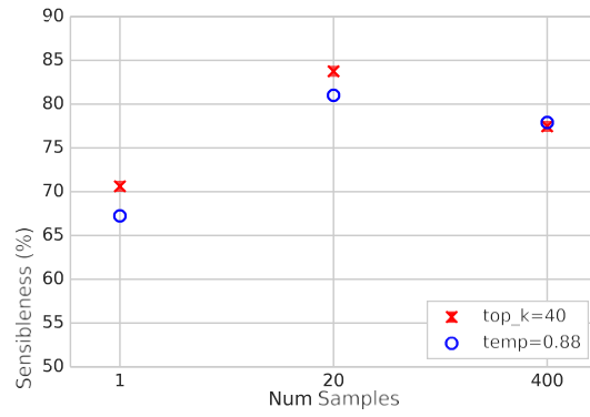
Figure 7: Static sensibleness over number of sampled responses for top- k and sampling with temperature.
