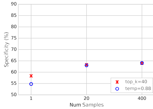
Figure 8: Static specificity over number of sampled responses for top- k and sampling with temperature.
