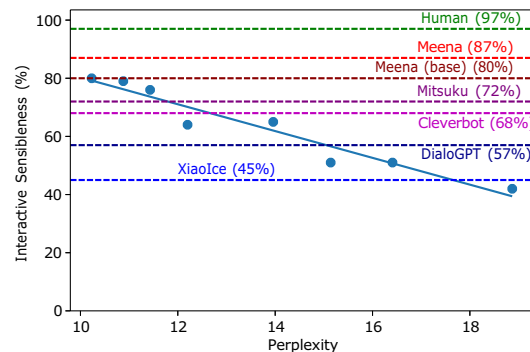
Figure 3: Interactive sensibleness vs perplexity.
